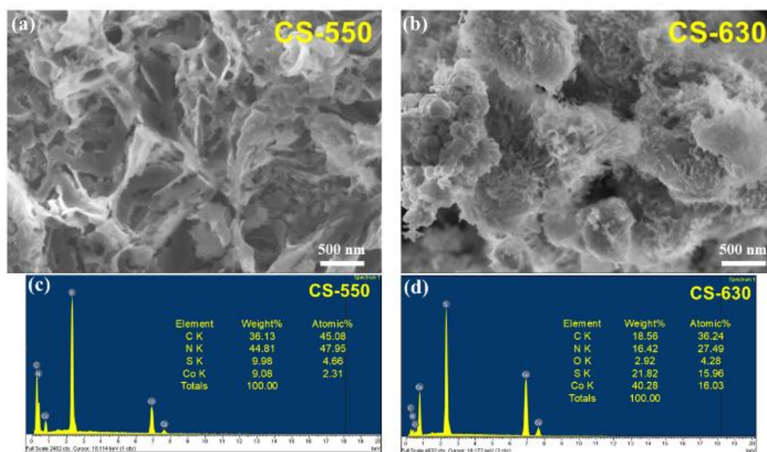
Fig. 2: SEM images and EDS spectra of CS-550 and CS-630
