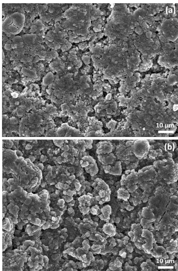
Fig. 6: SEM images of the CS-550 (a) and CS-630 (b) anode after 10 cycles.
