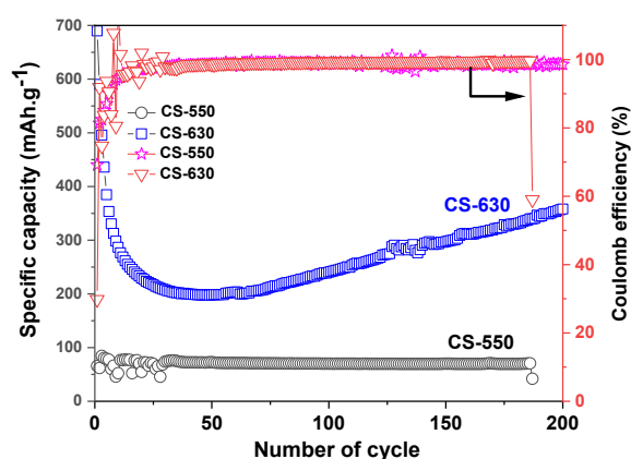
Fig. 4: Specific capacity and Coulombic efficiency of the CS-550 and CS-630 electrodes.
