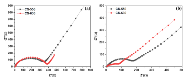
Fig. 5: EIS spectra of the CS-550 and CS-630 electrodes at the pristine state (a) and the 50 th cycle (b).
