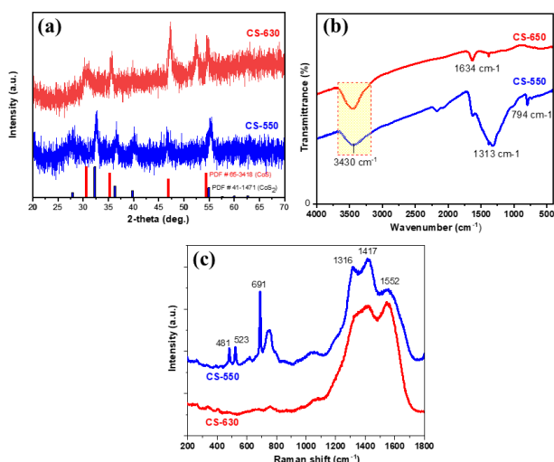
Fig. 1: XRD patterns (a), IR (b) and Raman (c) spectra of CS-550 and CS-630 materials.
