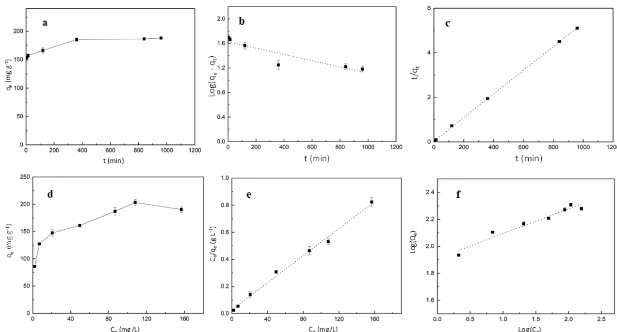
Fig. 3: Adsorption kinetics on BASP (a), pseudo-first order model linear plot (b), pseudo-second order model linear plot (c); Isotherm of MB adsorption on BASP (d), Langmuir isotherm model (e), Freundlich isotherm model linear plot (f) for MB adsorption onto BASP.
