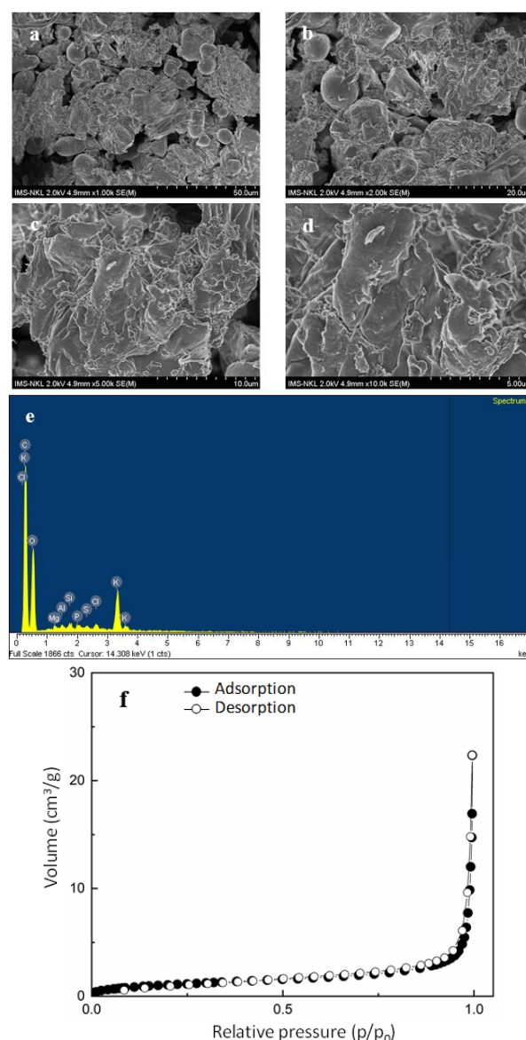
Fig. 2: SEM images at varying magnification (a-d), EDX spectrum (e), and N 2 adsorption-desorption isotherm (f) of BASP.
