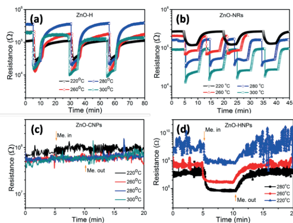
Figure 6: The resistance behavior of ZnO-H (a), ZnO-NRs (b), ZnO-CNPs (c) and ZnO-HNPs (d) based sensors upon exposure to 1.03% methanol vapor in dry air at different working temperatures.
